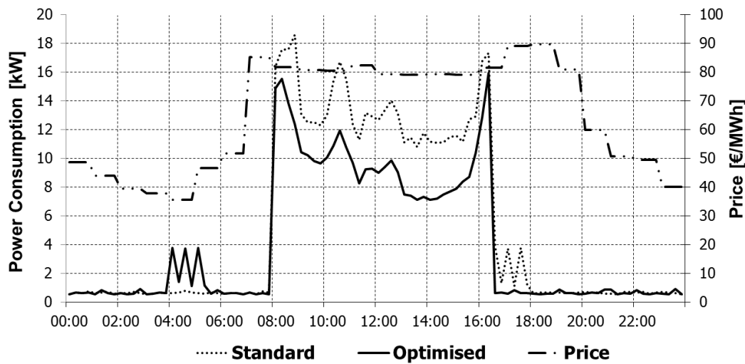
Fig. 5: Optimisation Variant A winter day (Data from EXAA 2011 and Inschlag 2011)
