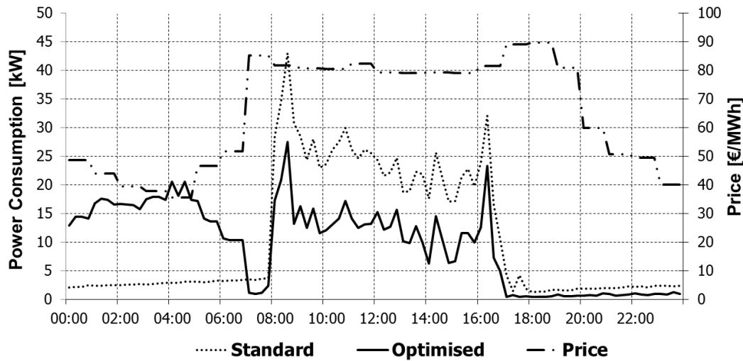
Fig. 7: Optimisation Variant B winter day (Data from EXAA 2011 and Inschlag 2011)
