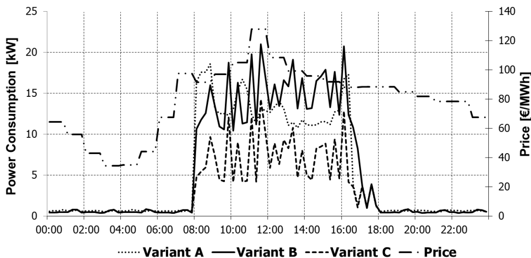
Fig. 2: Standard load curves on a summer day (Data from EXAA 2011 and Inschlag 2011)
