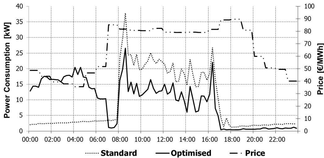
Fig. 9: Optimisation Variant B winter day (Data from EXAA 2011 and Inschlag 2011)
