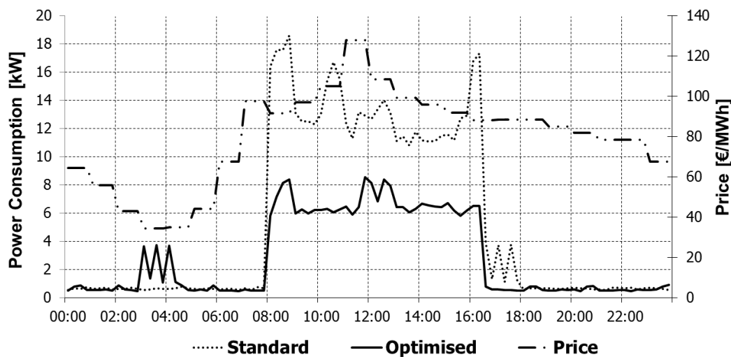
Fig. 4: Optimisation Variant A summer day (Data from EXAA 2011 and Inschlag 2011)
