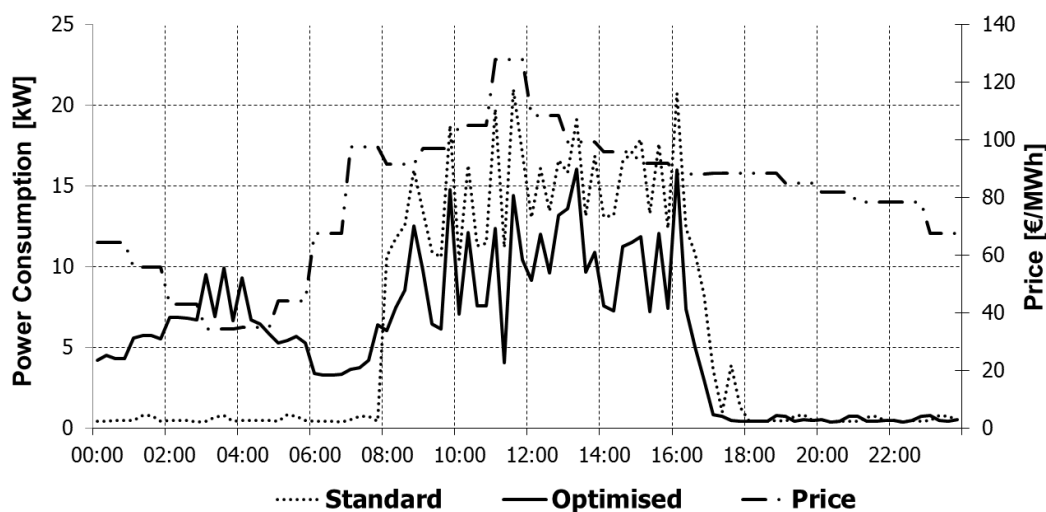
Fig. 6: Optimisation Variant B summer day (Data from EXAA 2011 and Inschlag 2011)
