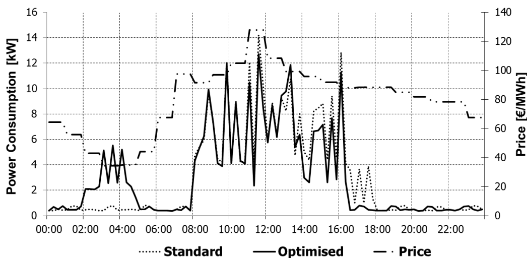
Fig. 8: Optimisation Variant C summer day (Data from EXAA 2011 and Inschlag 2011)
