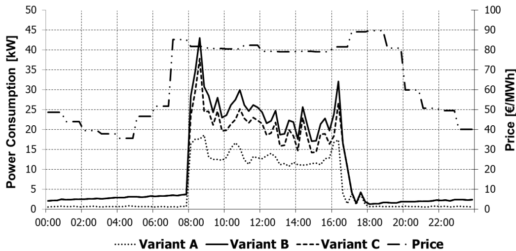
Fig. 3: Standard load curves on a winter day (Data from EXAA 2011 and Inschlag 2011)
