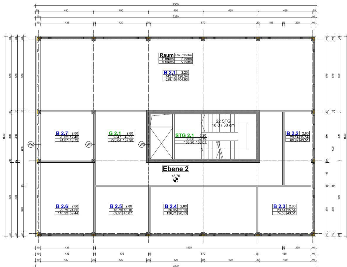
Fig. 1: Floor plan of the standard office building (Stumpf, 2011)
