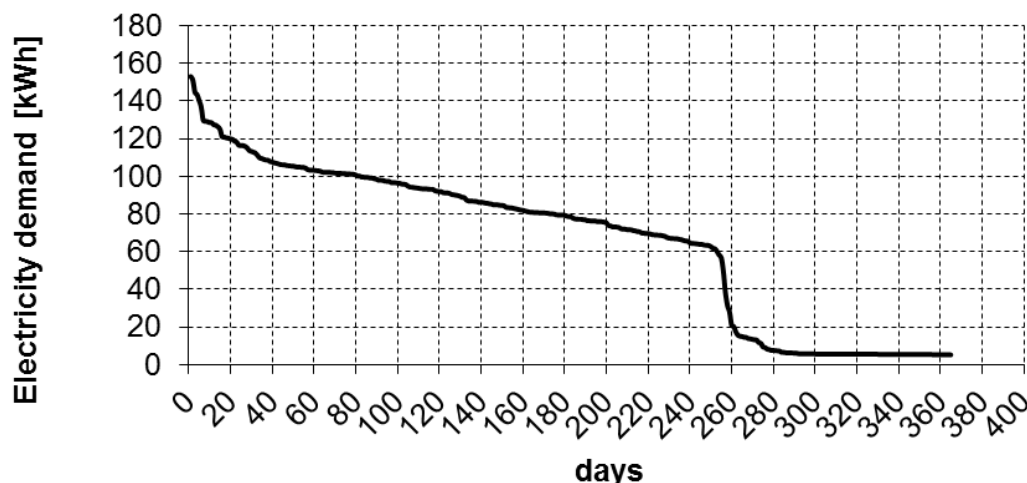
Fig. 9: Optimisation Variant B winter day (Data from EXAA 2011 and Inschlag 2011)
